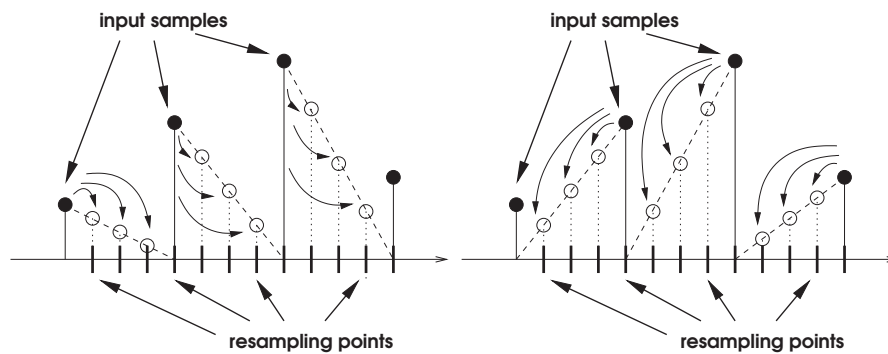
Figure 21.3: Distributing the contributions of all “left-hand” (a), and all “right-hand” (b) neighbors, when using a tent filter.
