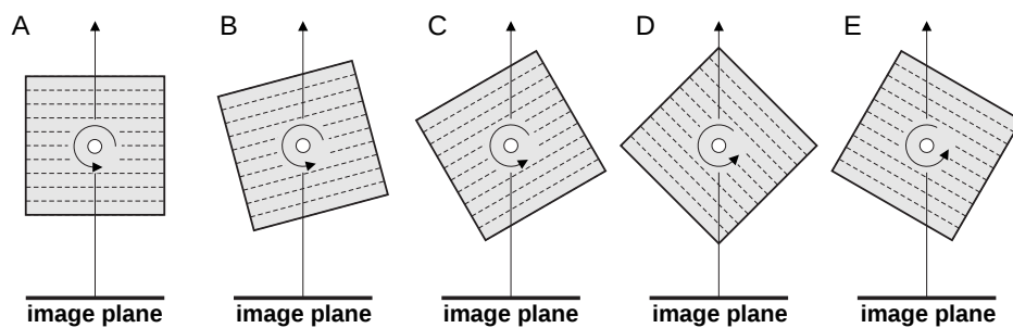
Figure 3.4: Switching the slice stack of object-aligned slices according to the viewing direction. Between image (C) and (D) the slice stack used for rendering has been switched.
