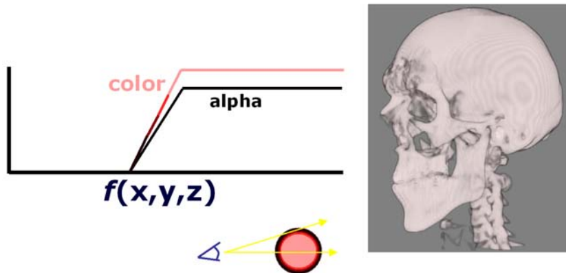
Figure 19.2: Faux shading. Modify the transfer function to create silhouette edges.
