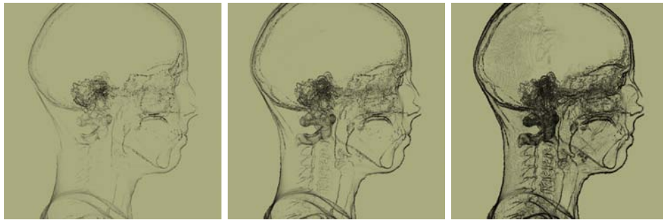
Figure 32.2: Simple contour enhancement based on gradient magnitude and angle between view and local gradient direction. The gradient magnitude windowing function g(\cdot) is an easy way to control contour appearance. These images simply use three different window settings.
