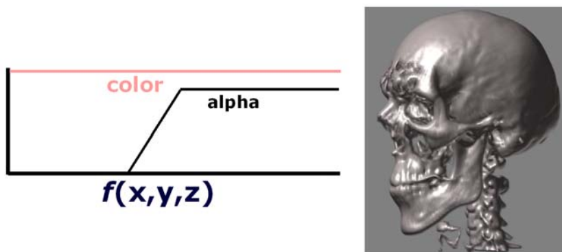
Figure 19.3: Surface shading.
