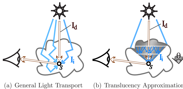
Figure 18.6: On the left is the general case of direct illumination I_d and scattered indirect illumination I_i . On the right is a translucent shading model which includes the direct illumination I_d and approximates the indirect, I_i , by blurring within the shaded region. Theta is the angle indicated by the shaded region.
