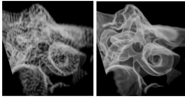
Figure 15.1: Pre-classification (left) versus post-classification (right)
