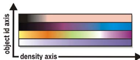
Figure 36.3: Instead of multiple one-dimensional transfer functions for different objects, we are using a single global two-dimensional transfer function texture. After determining the object ID for the current fragment via filtering, the fragment shader appropriately samples this texture with (density, object\_id) texture coordinates.
