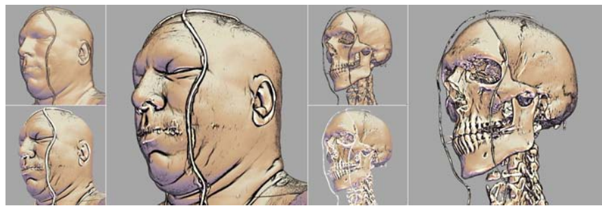
Figure 15.3: Using curvature and shape measures as axes of the transfer function. The upper small images show silhouette edges, the lower small images show ridge valley emphasis, and the large images show these combined into the final illustration. Images courtesy of Gordon Kindlman, use by permission.
