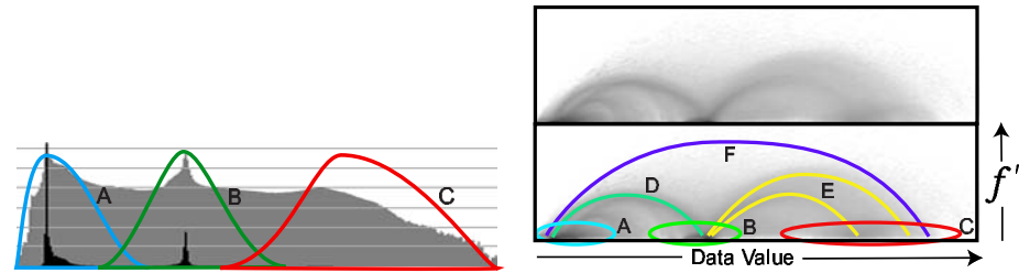
(a) A 1D histogram. The black region represents the number of data value occurrences on a linear scale, the grey is on a log scale. The colored regions (A,B,C) identify basic materials. (b) A log-scale 2D joint histogram. The lower image shows the location of materials (A,B,C), and material boundaries (D,E,F).
